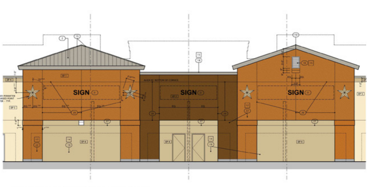
ENLARGED BACK MID-COURT ELEVATION TYPE 1 3/16" = 1'-0"
