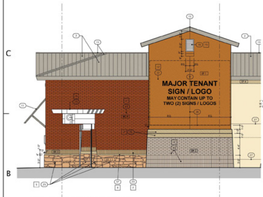
ENLARGED SOUTH ELEVATION 3/16" = 1'-0"
