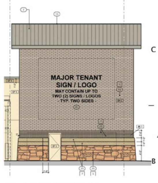
ENLARGED SOUTH ELEVATION 3/16" = 1'-0"
