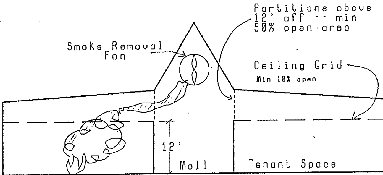
Vertical Section
